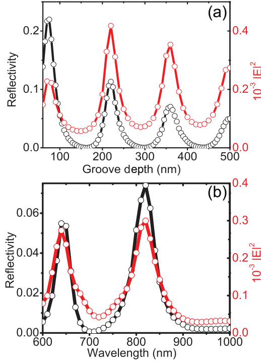
Figure 6.3: FDTD calculations (black) of the reflectivity for surface plasmons incident perpendicularly onto a groove structured into a gold surface as a function of groove depth. Electric field intensity integrated over the area A of the groove as calculated from BEM (red). (a) Calculations as a function of groove depth at a free-space wavelength of 640 nm for a 25 nm wide groove; (b) Calculations as a function of wavelength for a 500 nm deep, 25 nm wide groove.
