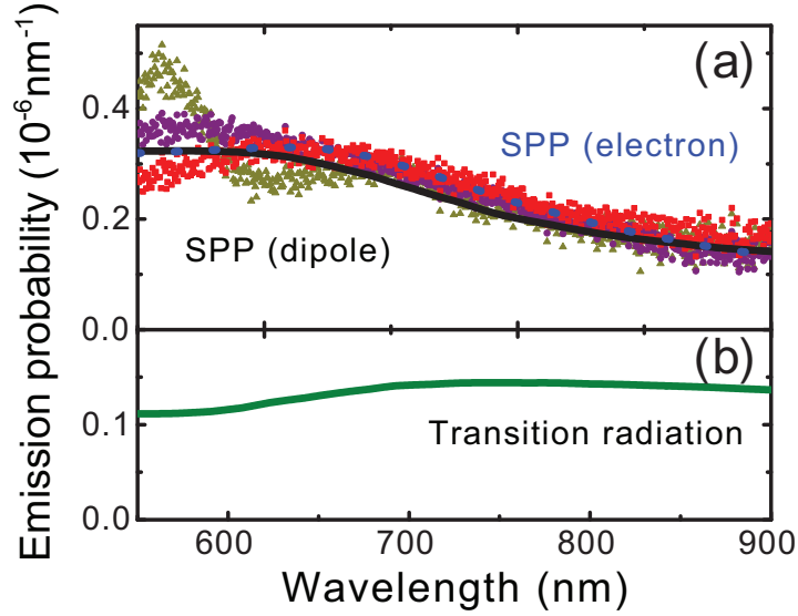
Figure 3.3: (a) Spectrum of surface plasmon polaritons on single-crystal gold excited by 30 keV electrons and integrated over a line next to gratings with three different grating pitches [ a = 300 nm - yellow triangles, 400 nm - violet dots, 500 nm - red squares]. The solid lines show calculated spectra for SPPs generated by a 30 keV electron impinging on the surface (blue, dashed) and by a dipole positioned at the surface (black, solid). (b) Calculated transition radiation spectrum for 30 keV electrons on Au.
