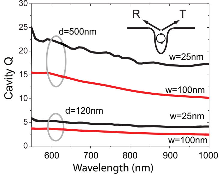
Figure 6.6: Cavity quality factor Q for 25 nm (black) and 100 nm (red) wide grooves with depths of 120 nm and 500 nm. Q was calculated from FDTD calculations of the groove end reflection coefficients and propagation losses for MIM plasmons.
