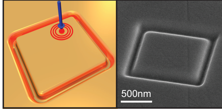
Figure 7.1: (a) Schematic of the structure under investigation. The electron beam is shown as a blue arrow that excites surface plasmons (b) Top-view SEM image of a 1 \times 1 \mu\text{m} box bounded by 120 nm deep grooves structured into the surface of a single-crystal gold pellet.
