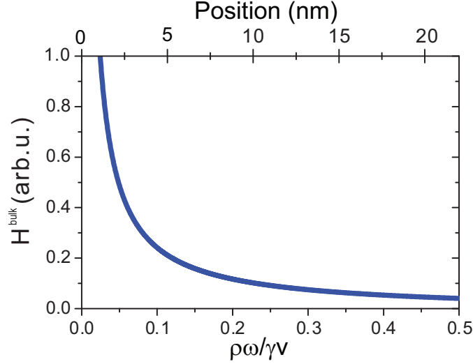
Figure 2.1: External magnetic field \mathbf{H}^{bulk} from Eqn. 2.11 as a function of radial distance from the electron trajectory. The top horizontal axis plots the corresponding positions for 30 keV electrons and a wavelength of 800 nm.
